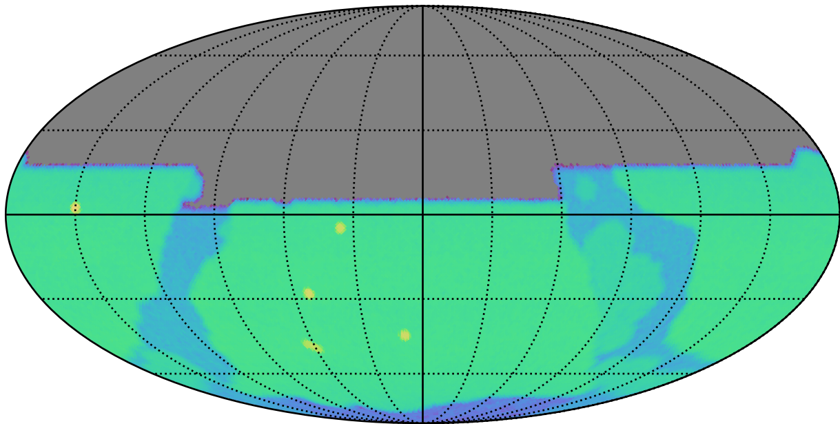
too_combined_s0.8_v3.4_10yrs y: SurfaceBrightLimit
