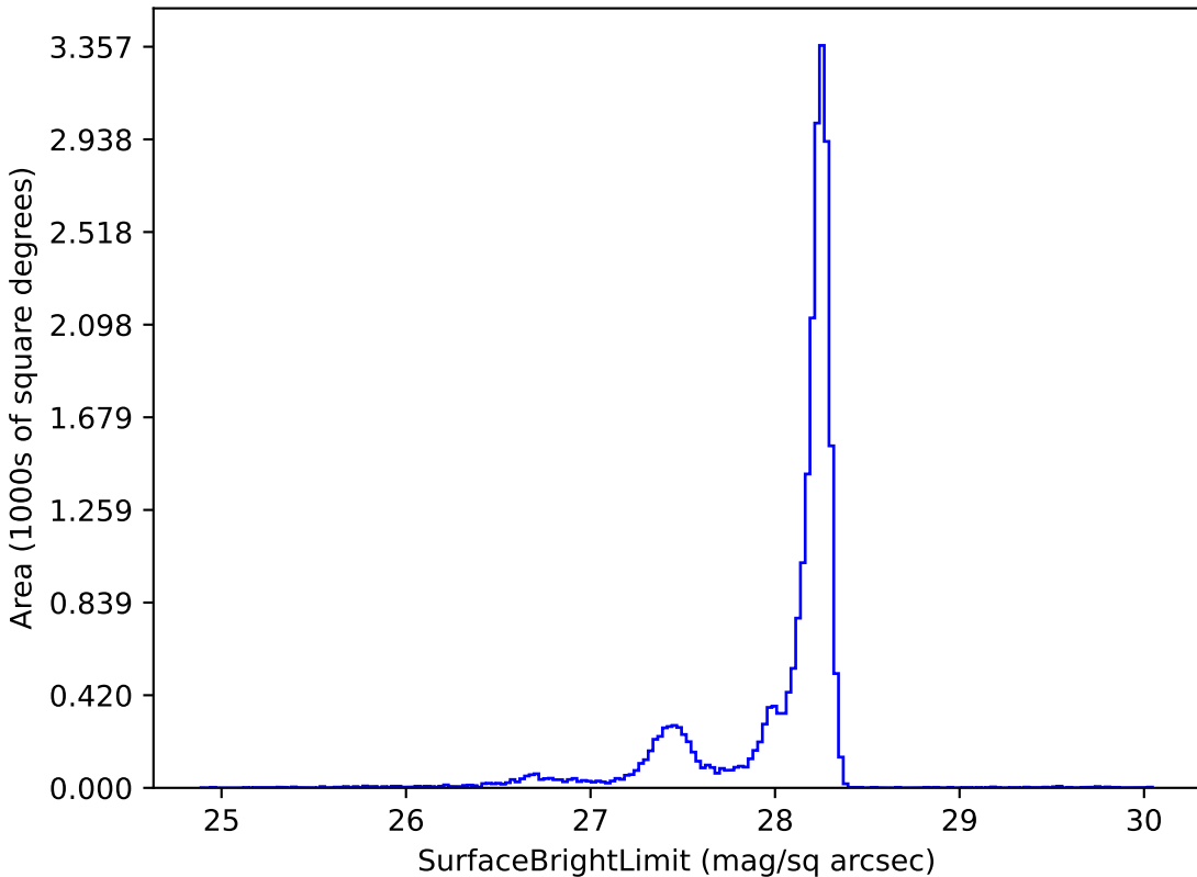
too_combined_s0.8_v3.4_10yrs y: SurfaceBrightLimit
