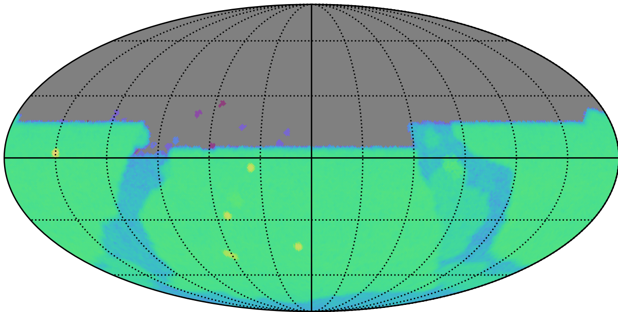
too_combined_s0.8_v3.4_10yrs u: SurfaceBrightLimit
