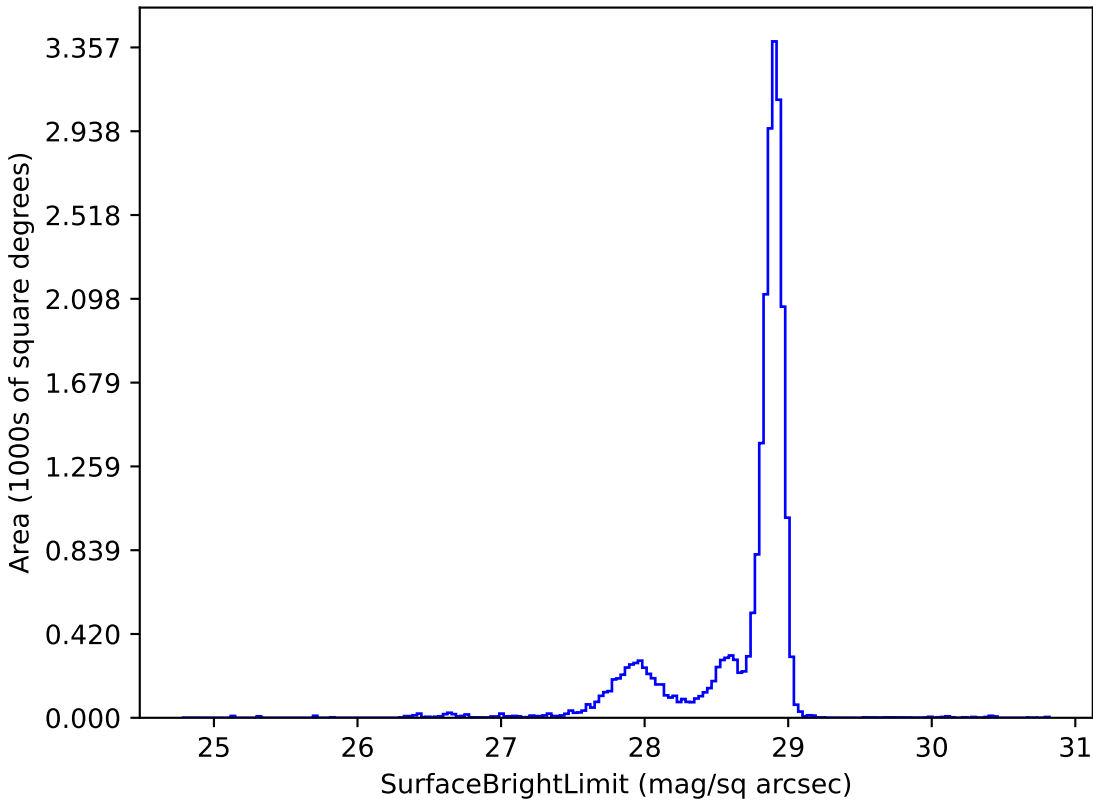
too_combined_s0.8_v3.4_10yrs u: SurfaceBrightLimit
