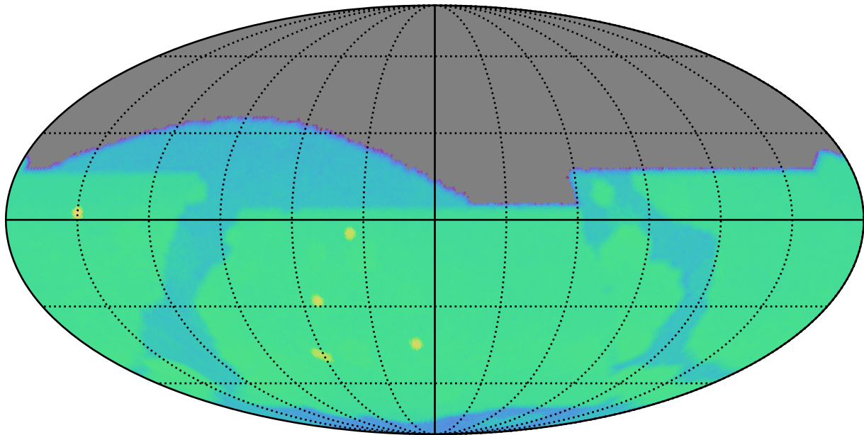
too_combined_s0.8_v3.4_10yrs r: SurfaceBrightLimit
