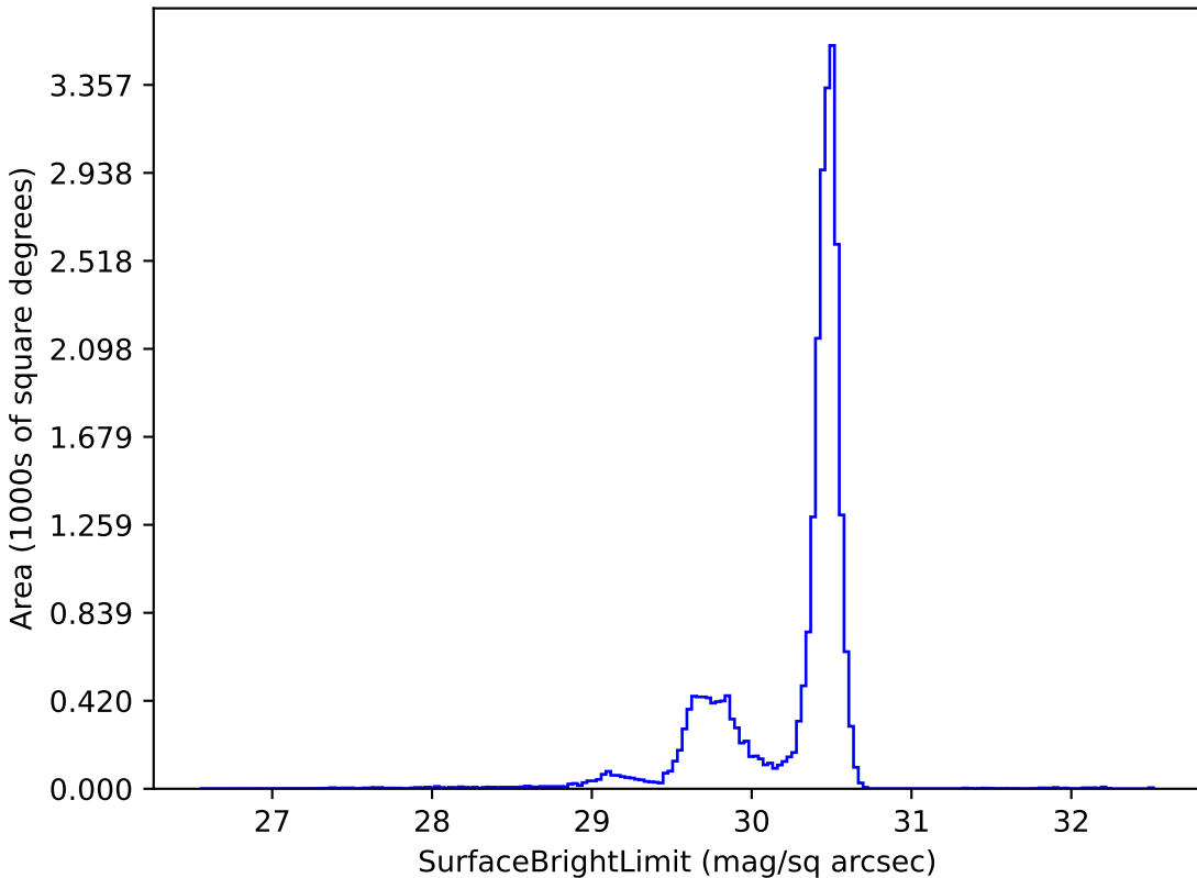
too_combined_s0.8_v3.4_10yrs r: SurfaceBrightLimit
