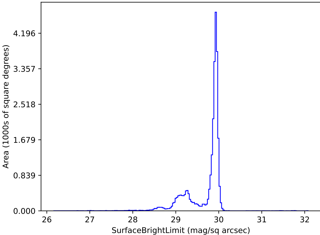
too_combined_s0.8_v3.4_10yrs i: SurfaceBrightLimit
