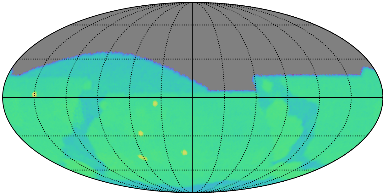
too_combined_s0.8_v3.4_10yrs g: SurfaceBrightLimit
