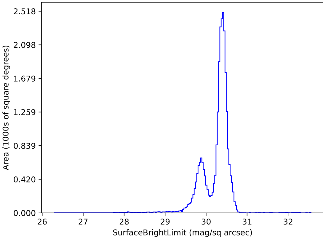
too_combined_s0.8_v3.4_10yrs g: SurfaceBrightLimit
