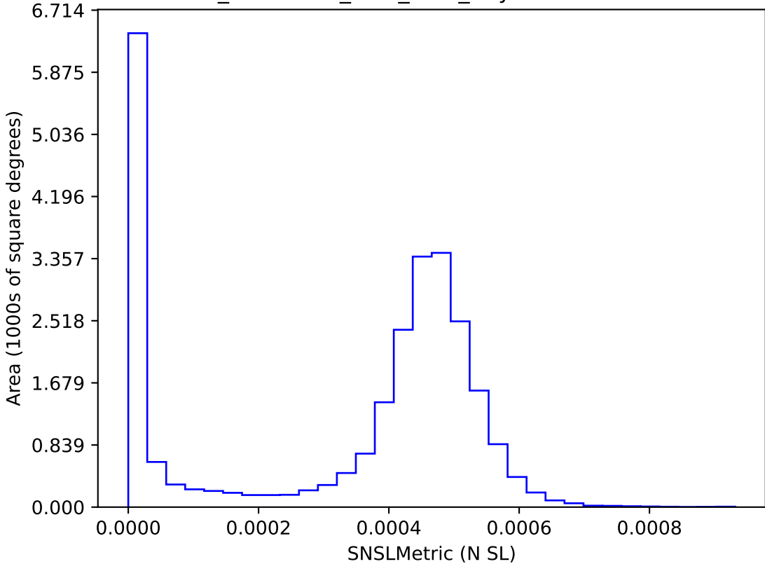
too_combined_s0.8_v3.4_10yrs : SNSLMetric
