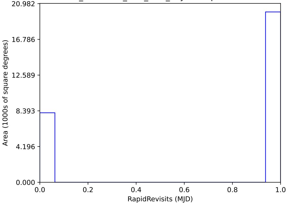
too_combined_s0.8_v3.4_10yrs : RapidRevisits
