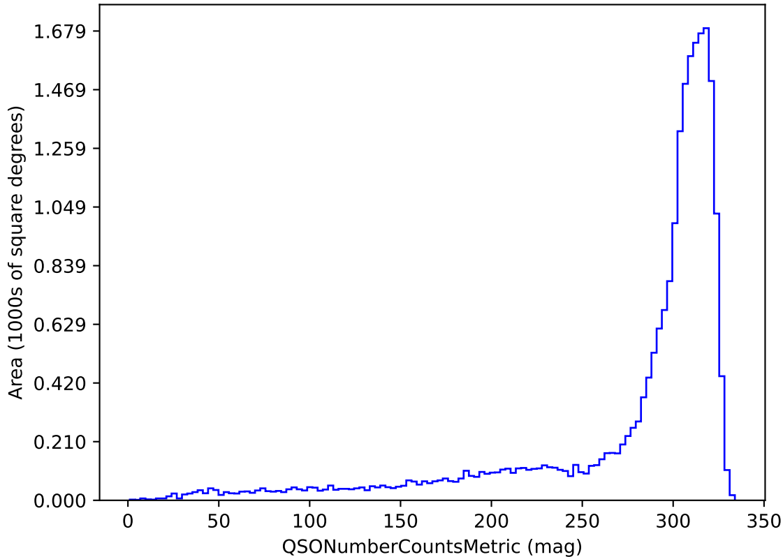
too_combined_s0.8_v3.4_10yrs u band and non-DD: QSONumberCountsMetric
