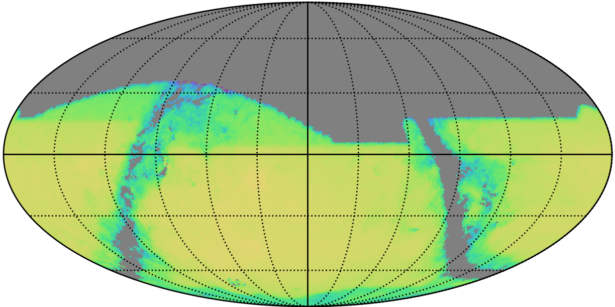
too_combined_s0.8_v3.4_10yrs r band and non-DD: QSONumberCountsMetric
