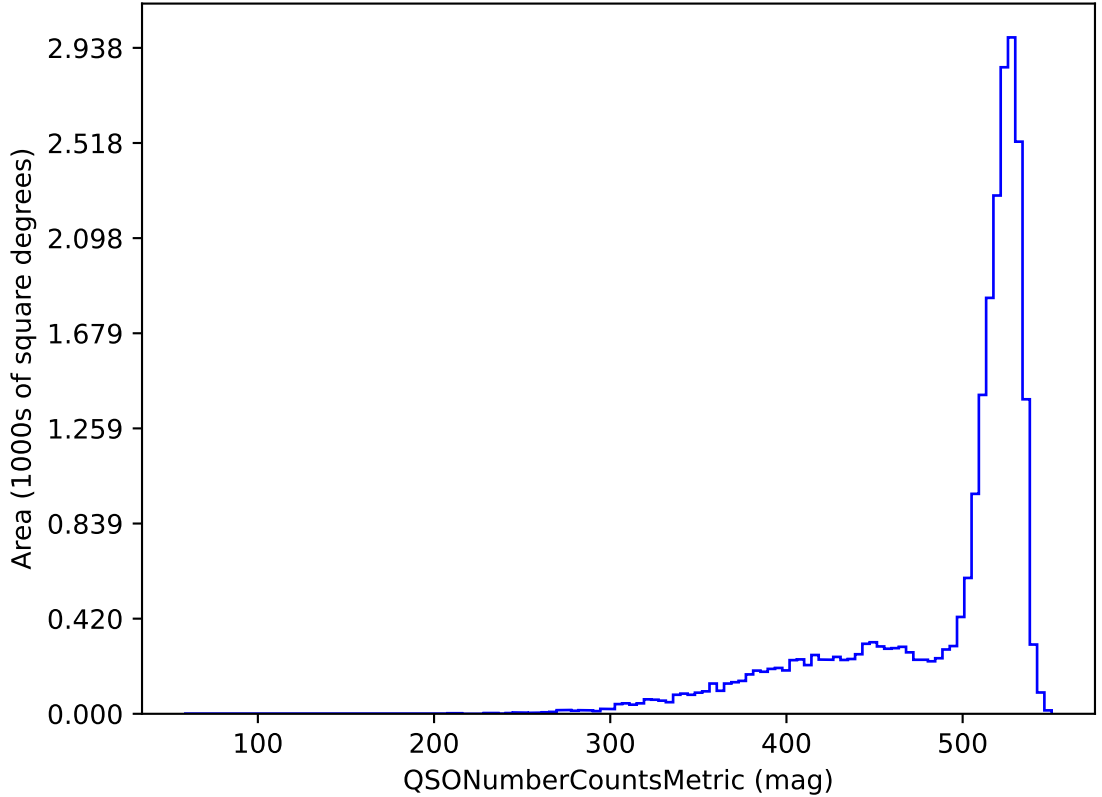
too_combined_s0.8_v3.4_10yrs r band and non-DD: QSONumberCountsMetric
