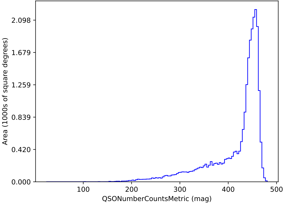
too_combined_s0.8_v3.4_10yrs g band and non-DD: QSONumberCountsMetric
