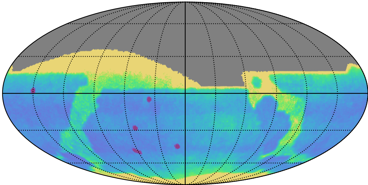
too_combined_s0.8_v3.4_10yrs : Proper Motion Uncert @ 24.0
