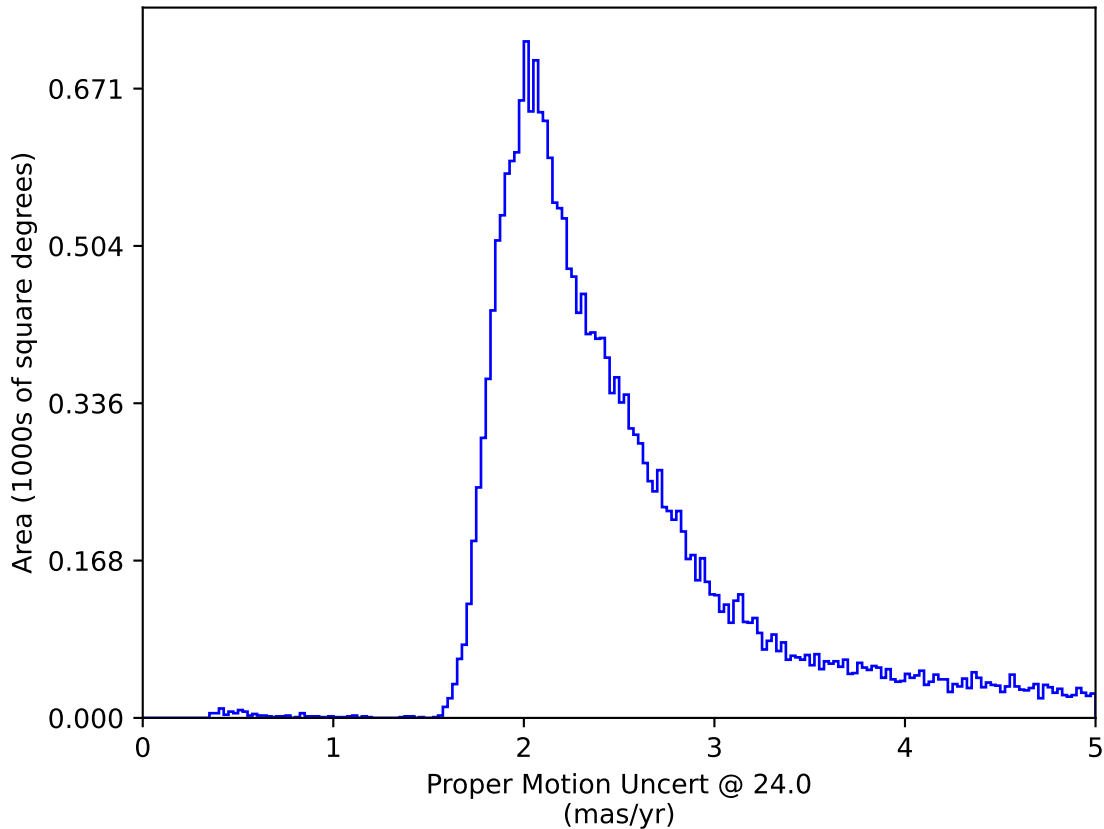
too_combined_s0.8_v3.4_10yrs : Proper Motion Uncert @ 24.0
