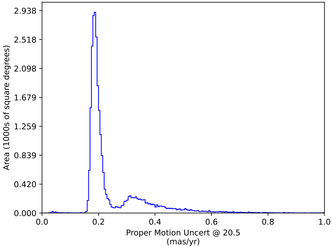
too_combined_s0.8_v3.4_10yrs : Proper Motion Uncert @ 20.5
