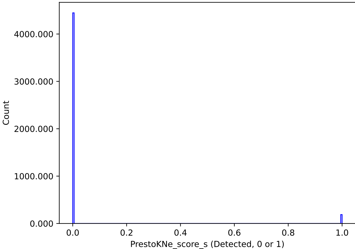
too_combined_s0.8_v3.4_10yrs : PrestoKNe_score_s
