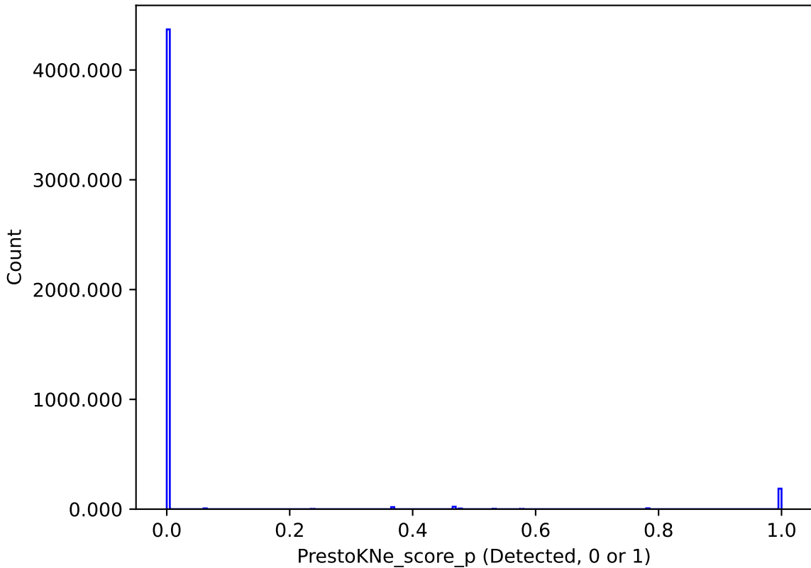
too_combined_s0.8_v3.4_10yrs : PrestoKNe_score_p
