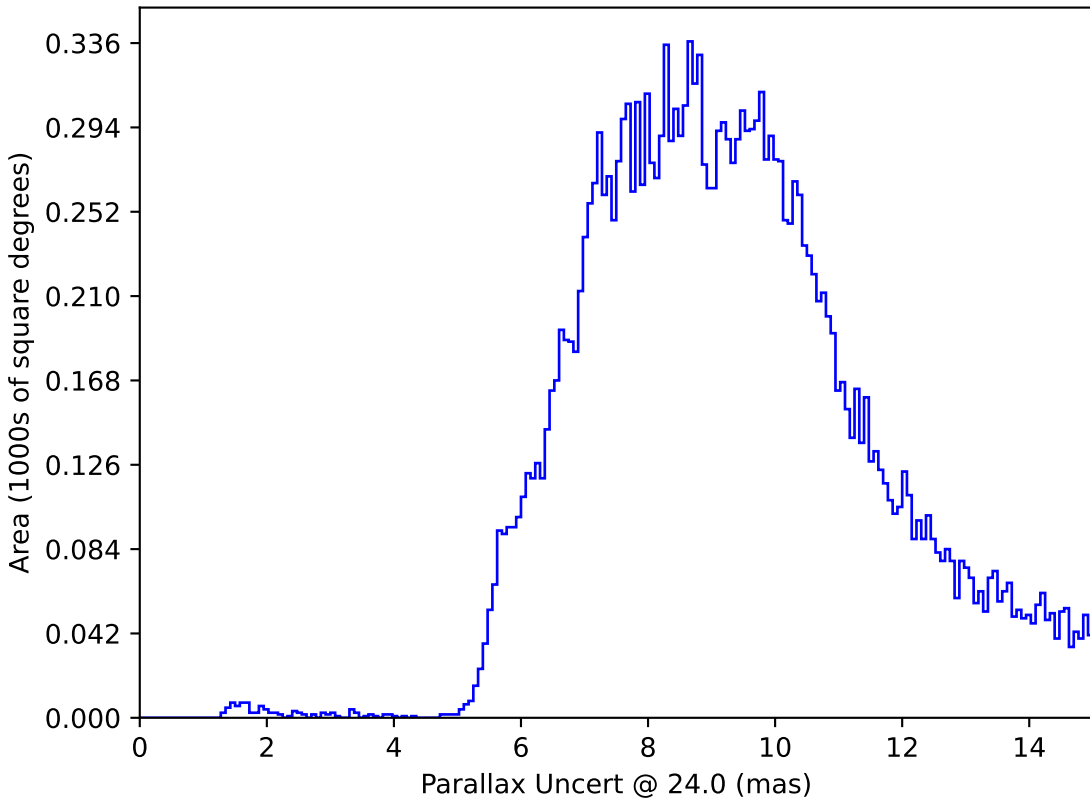
too_combined_s0.8_v3.4_10yrs : Parallax Uncert @ 24.0
