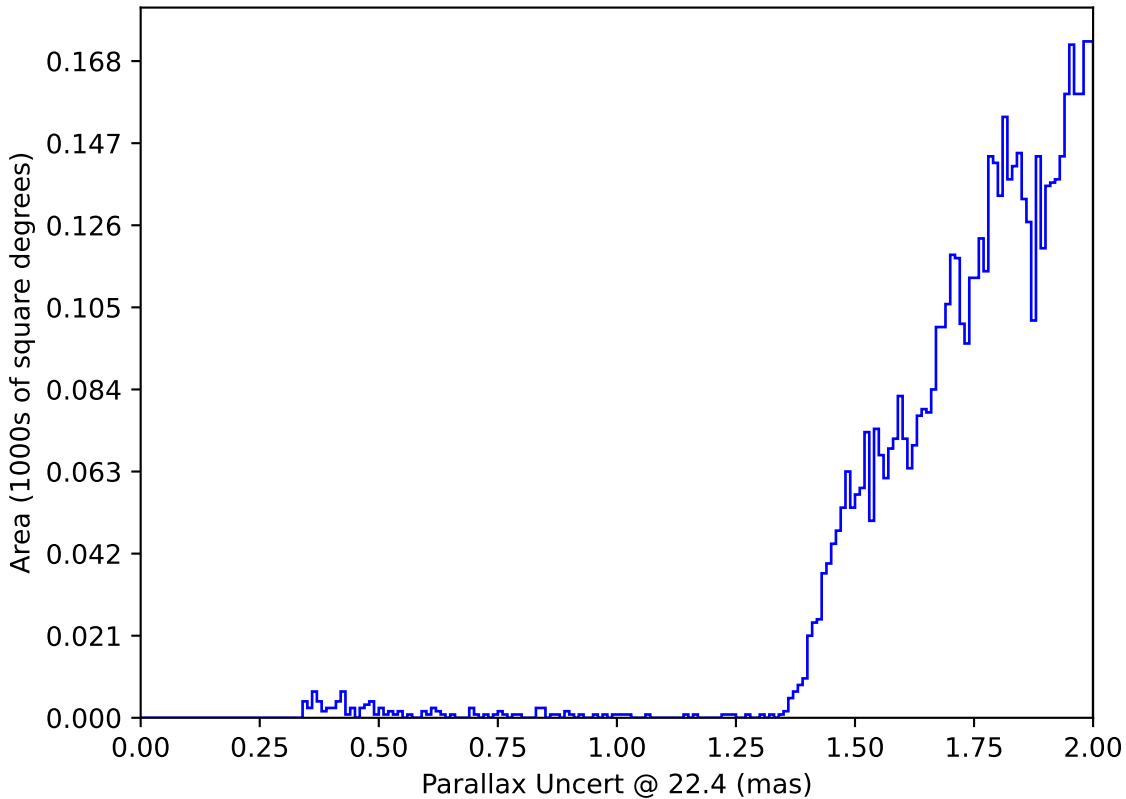
too_combined_s0.8_v3.4_10yrs : Parallax Uncert @ 22.4
