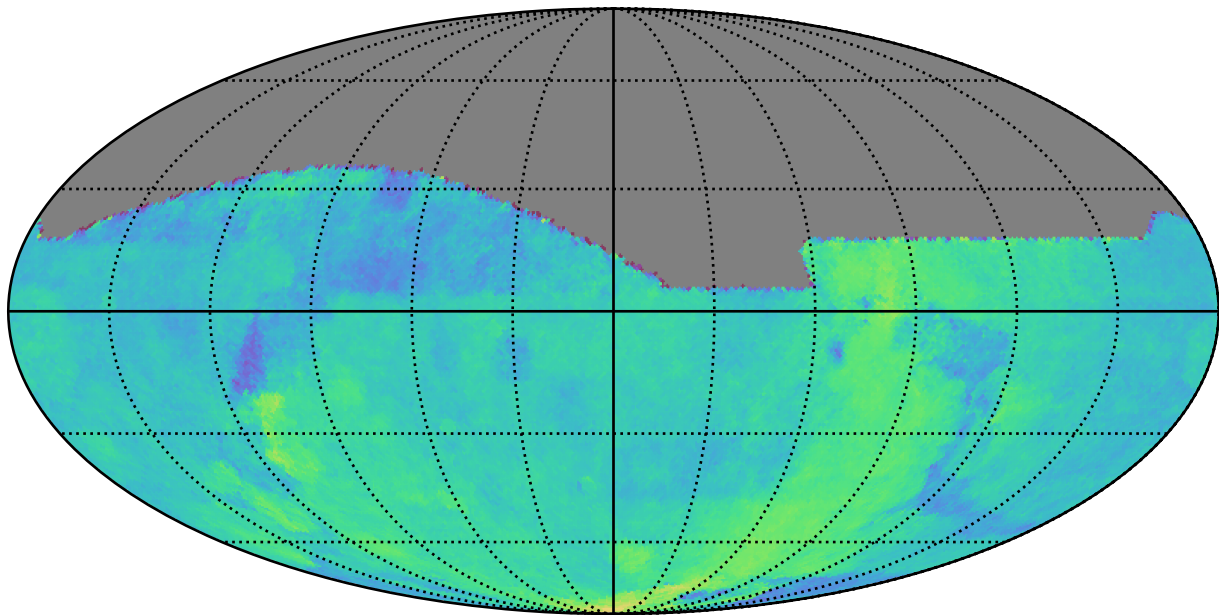
too_combined_s0.8_v3.4_10yrs : Parallax Coverage @ 24.0
