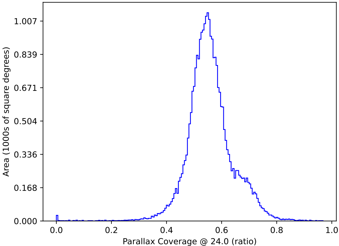
too_combined_s0.8_v3.4_10yrs : Parallax Coverage @ 24.0
