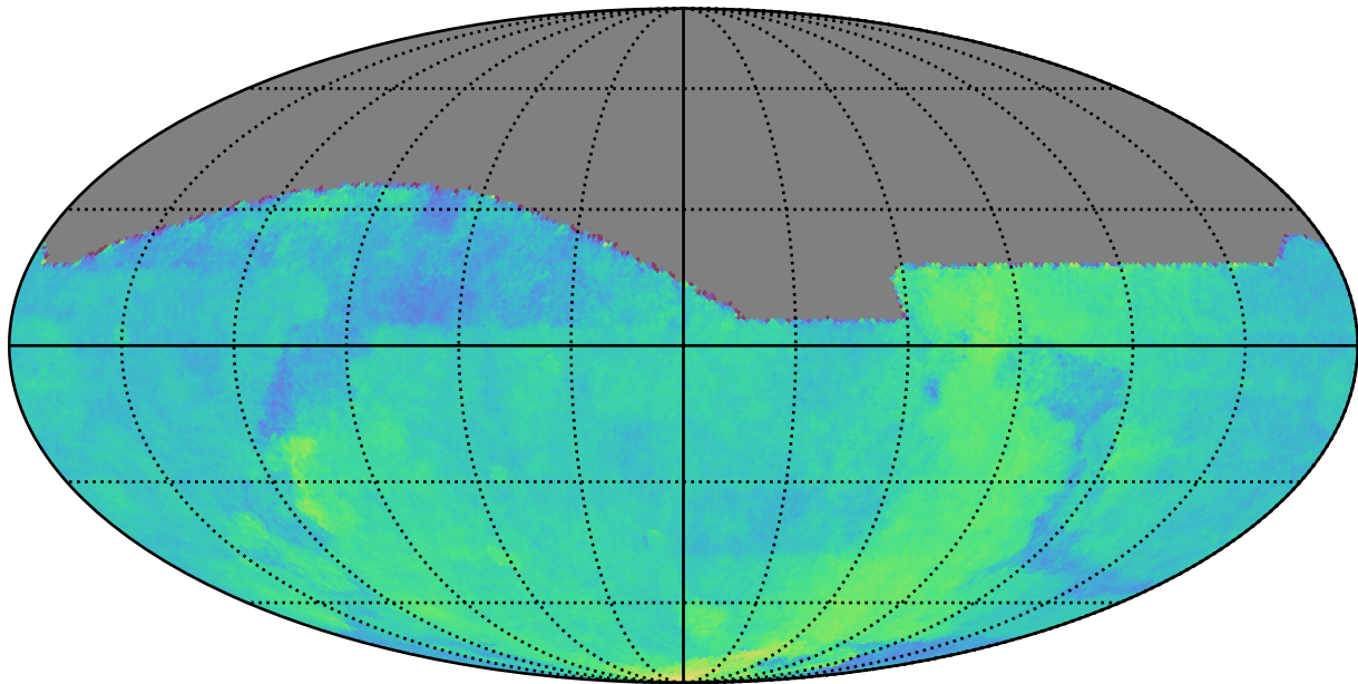
too_combined_s0.8_v3.4_10yrs : Parallax Coverage @ 22.4
