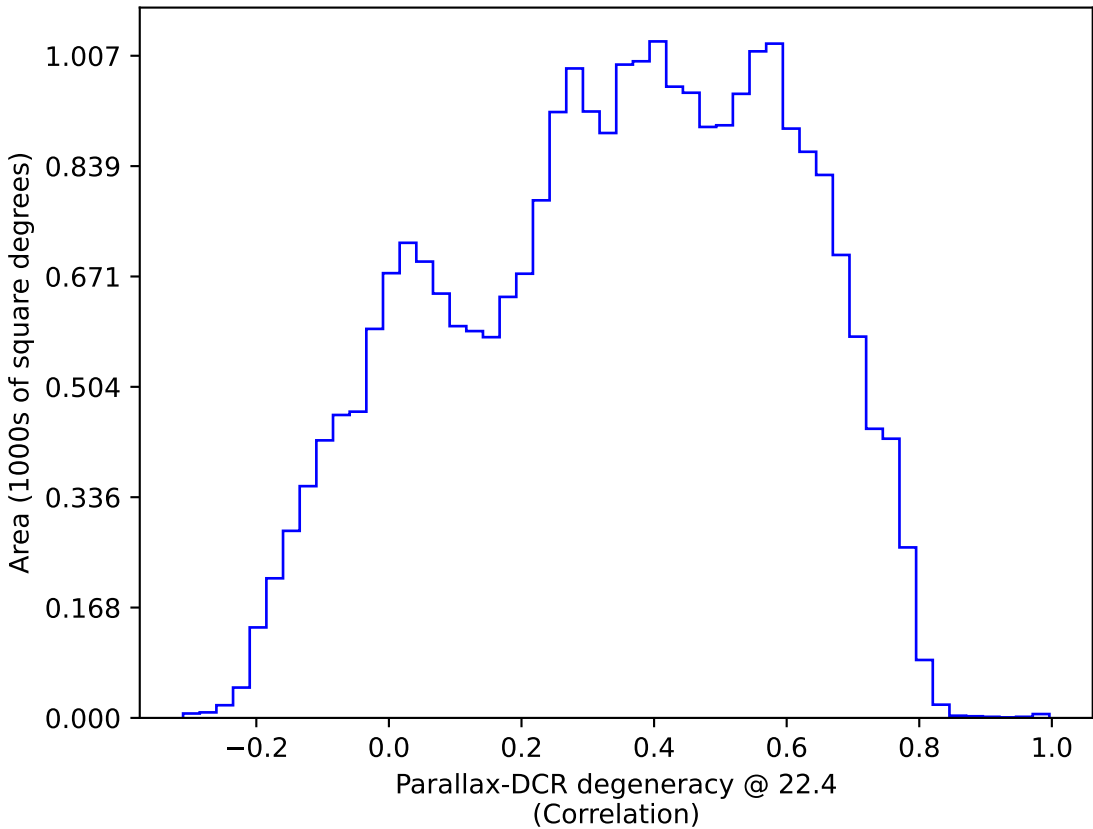
too_combined_s0.8_v3.4_10yrs : Parallax-DCR degeneracy @ 22.4
