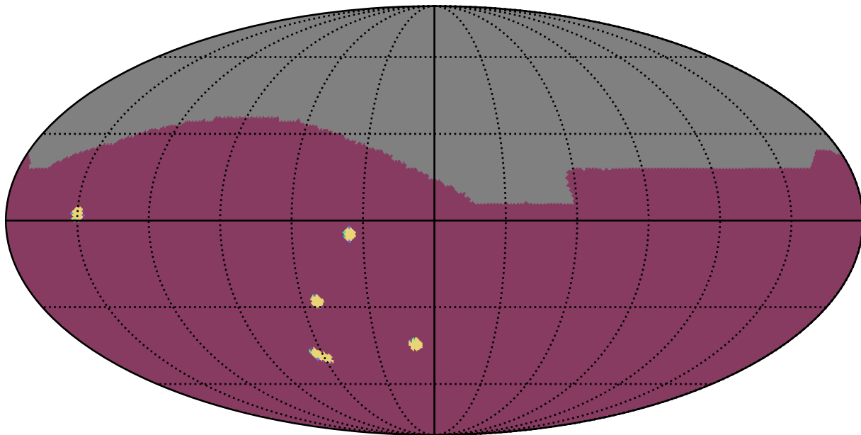
too_combined_s0.8_v3.4_10yrs : NumberOfQuickRevisits
