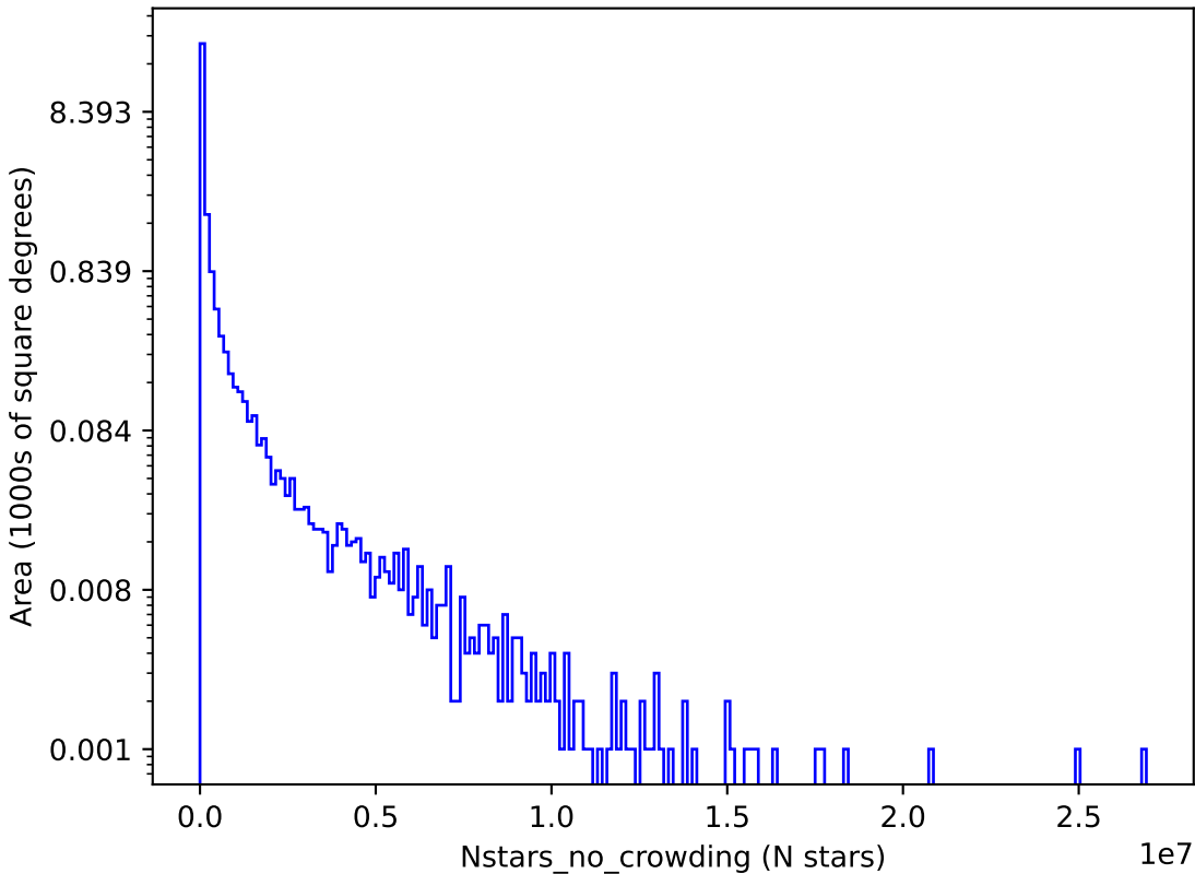
too_combined_s0.8_v3.4_10yrs z: Nstars_no_crowding
