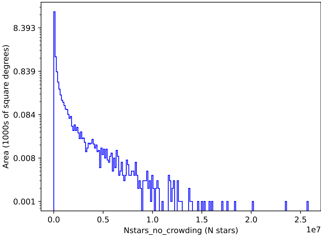
too_combined_s0.8_v3.4_10yrs y: Nstars_no_crowding
