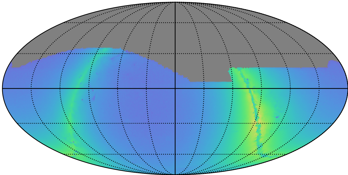
too_combined_s0.8_v3.4_10yrs r: Nstars_no_crowding
