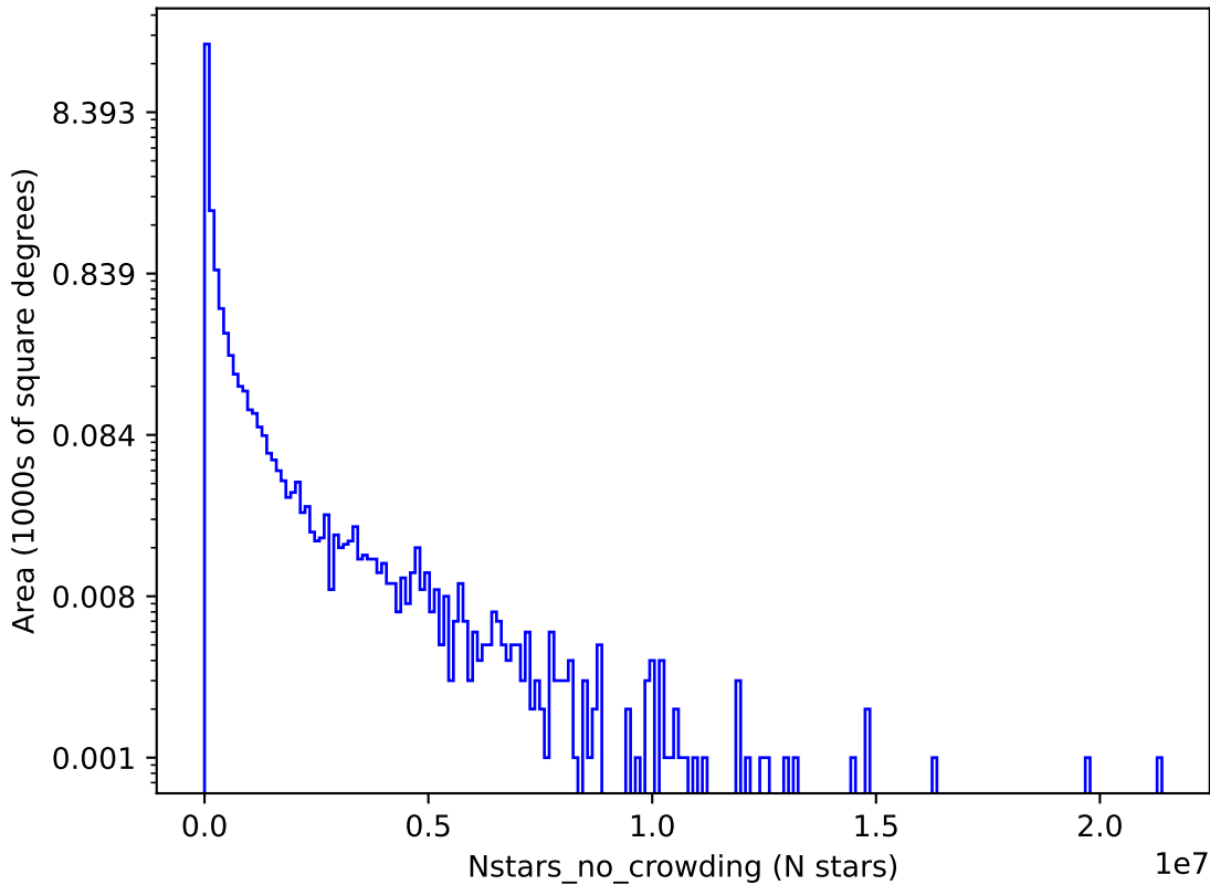
too_combined_s0.8_v3.4_10yrs r: Nstars_no_crowding
