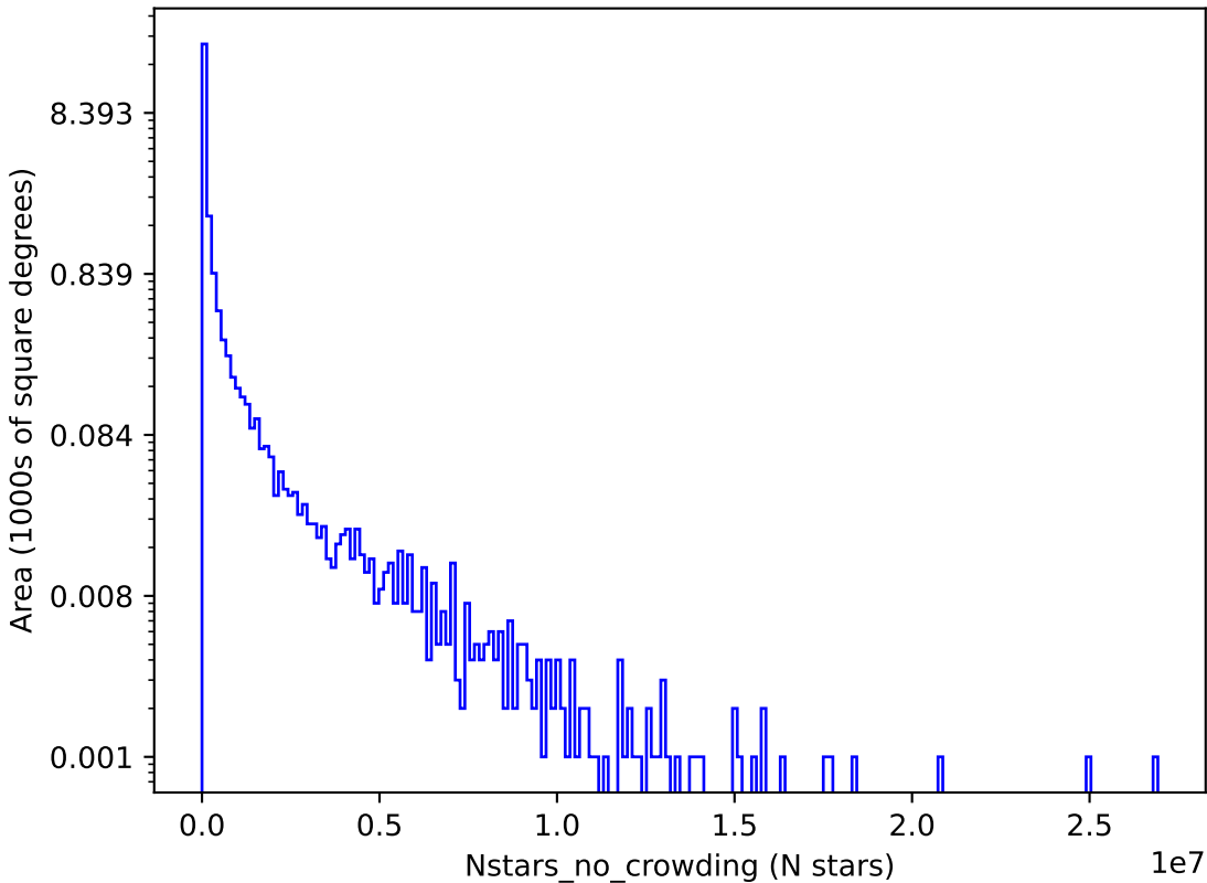
too_combined_s0.8_v3.4_10yrs i: Nstars_no_crowding
