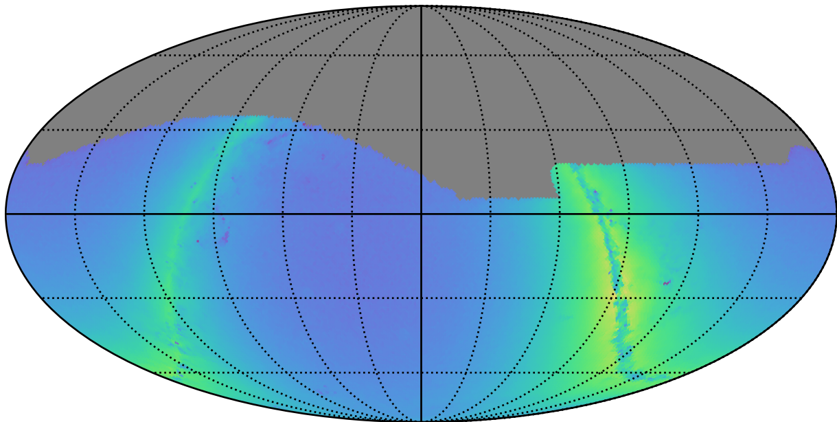
too_combined_s0.8_v3.4_10yrs g: Nstars_no_crowding
