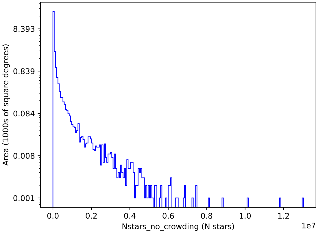
too_combined_s0.8_v3.4_10yrs g: Nstars_no_crowding
