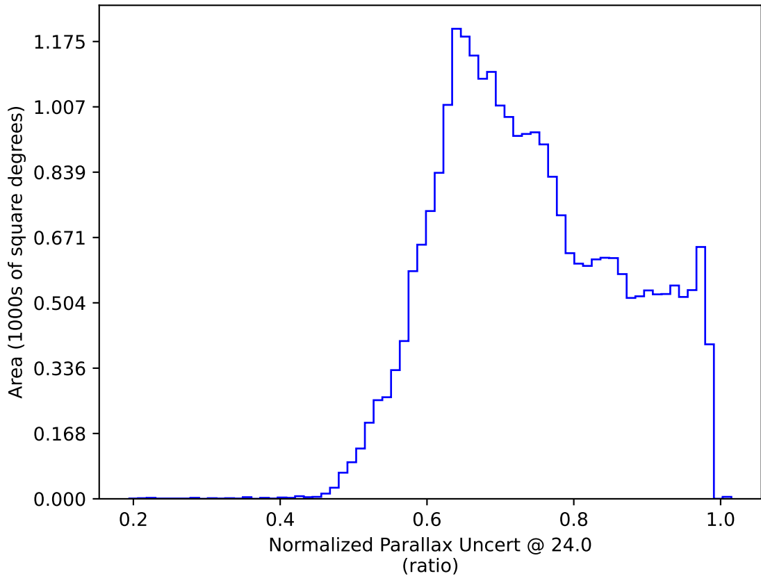
too_combined_s0.8_v3.4_10yrs : Normalized Parallax Uncert @ 24.0
