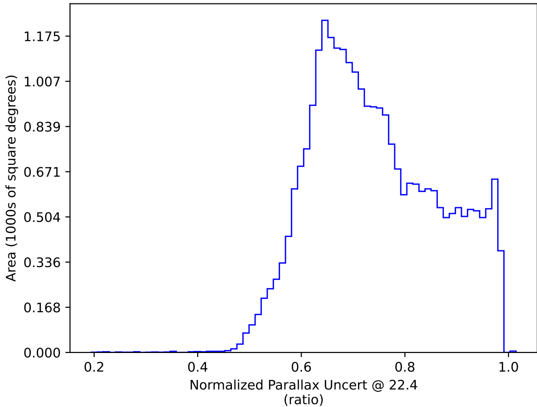
too_combined_s0.8_v3.4_10yrs : Normalized Parallax Uncert @ 22.4
