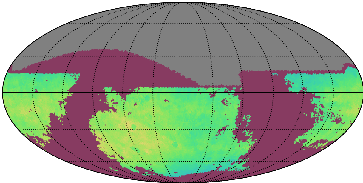
too_combined_s0.8_v3.4_10yrs i: NgalScale
