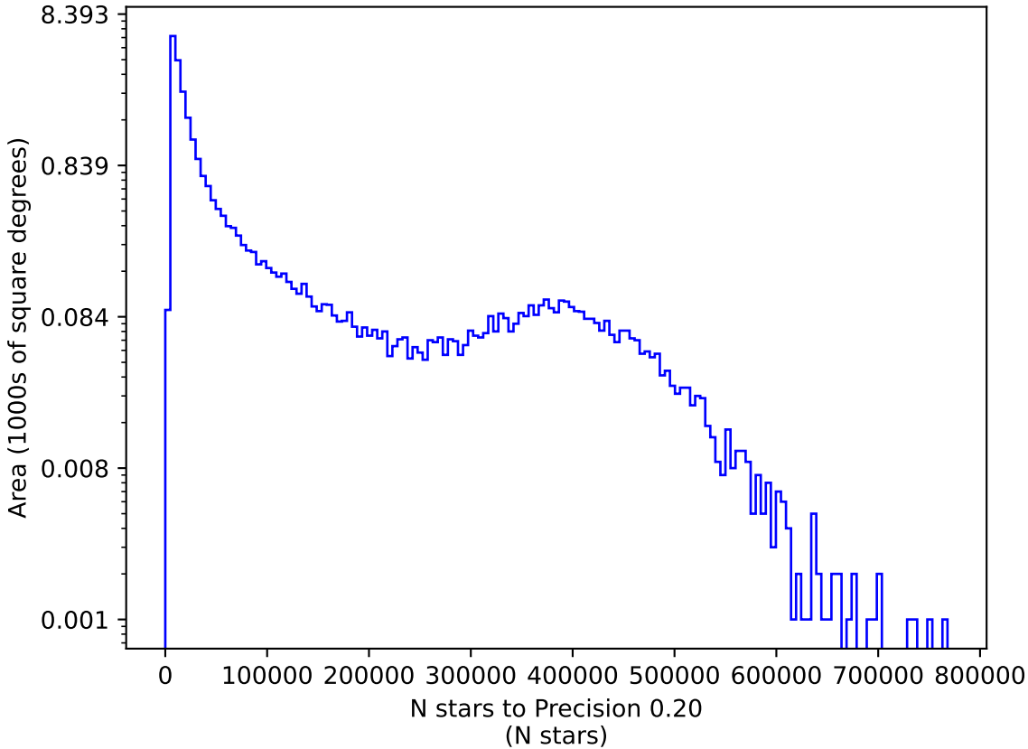
too_combined_s0.8_v3.4_10yrs z: N stars to Precision 0.20
