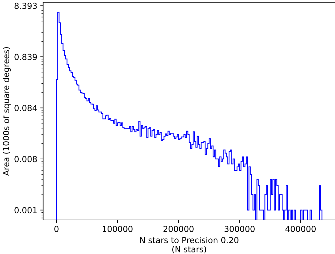
too_combined_s0.8_v3.4_10yrs u: N stars to Precision 0.20
