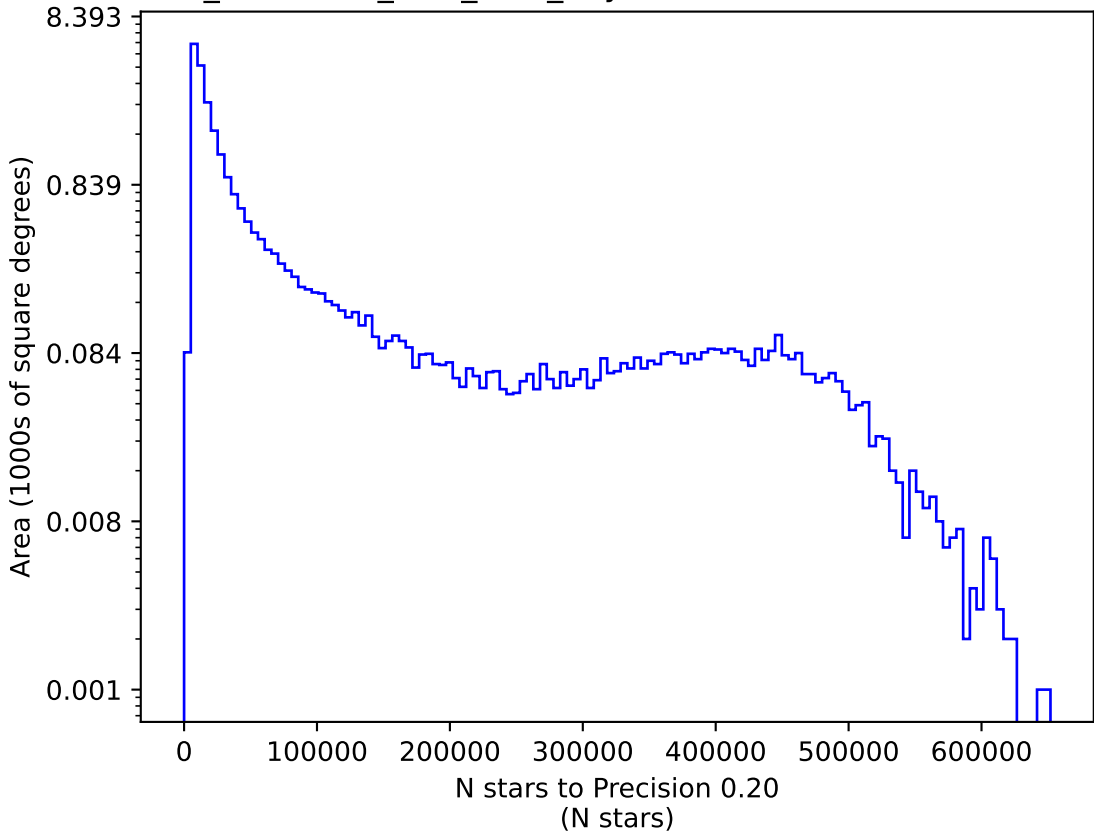
too_combined_s0.8_v3.4_10yrs i: N stars to Precision 0.20
