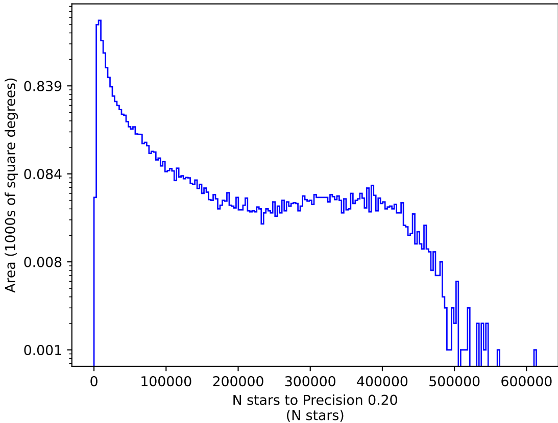
too_combined_s0.8_v3.4_10yrs g: N stars to Precision 0.20
