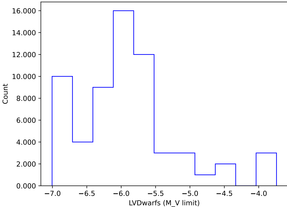
too_combined_s0.8_v3.4_10yrs gi: LVDwarfs
