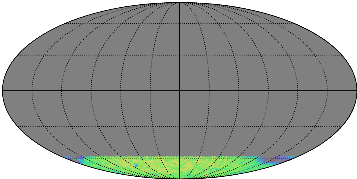
too_combined_s0.8_v3.4_10yrs gi SCP: LVDwarfs
