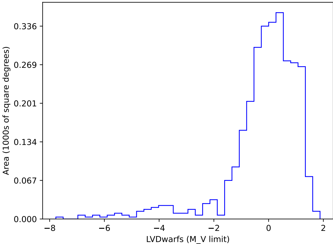
too_combined_s0.8_v3.4_10yrs gi SCP: LVDwarfs
