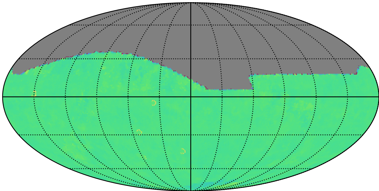
too_combined_s0.8_v3.4_10yrs z: Kuiper rotTelPos
