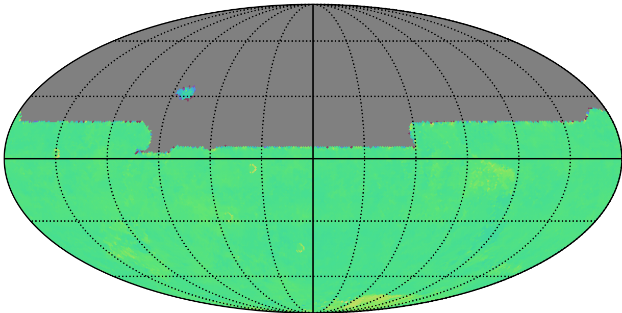
too_combined_s0.8_v3.4_10yrs y: Kuiper rotTelPos
