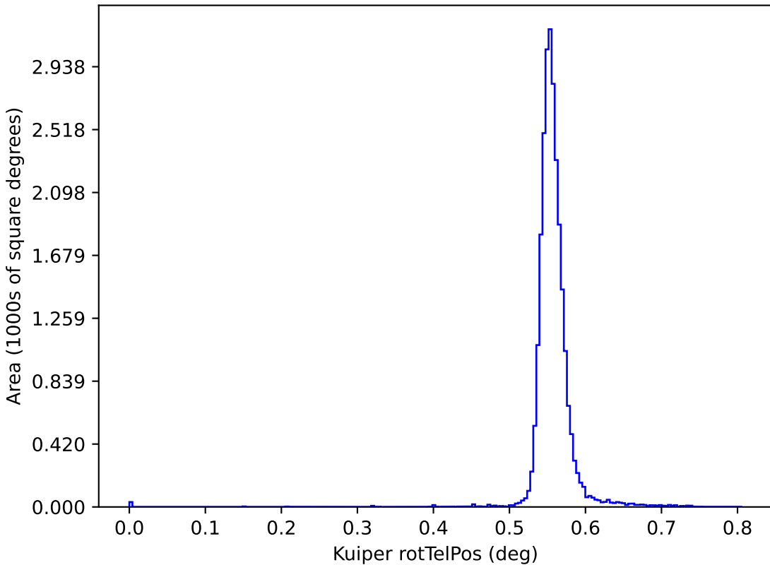
too_combined_s0.8_v3.4_10yrs y: Kuiper rotTelPos
