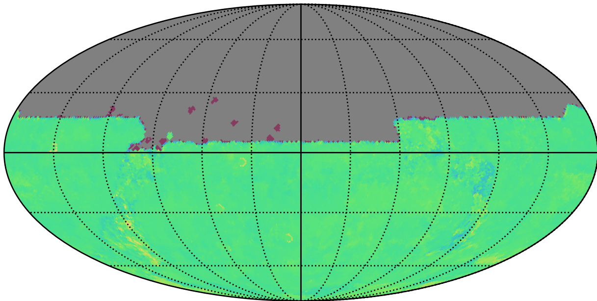
too_combined_s0.8_v3.4_10yrs u: Kuiper rotTelPos
