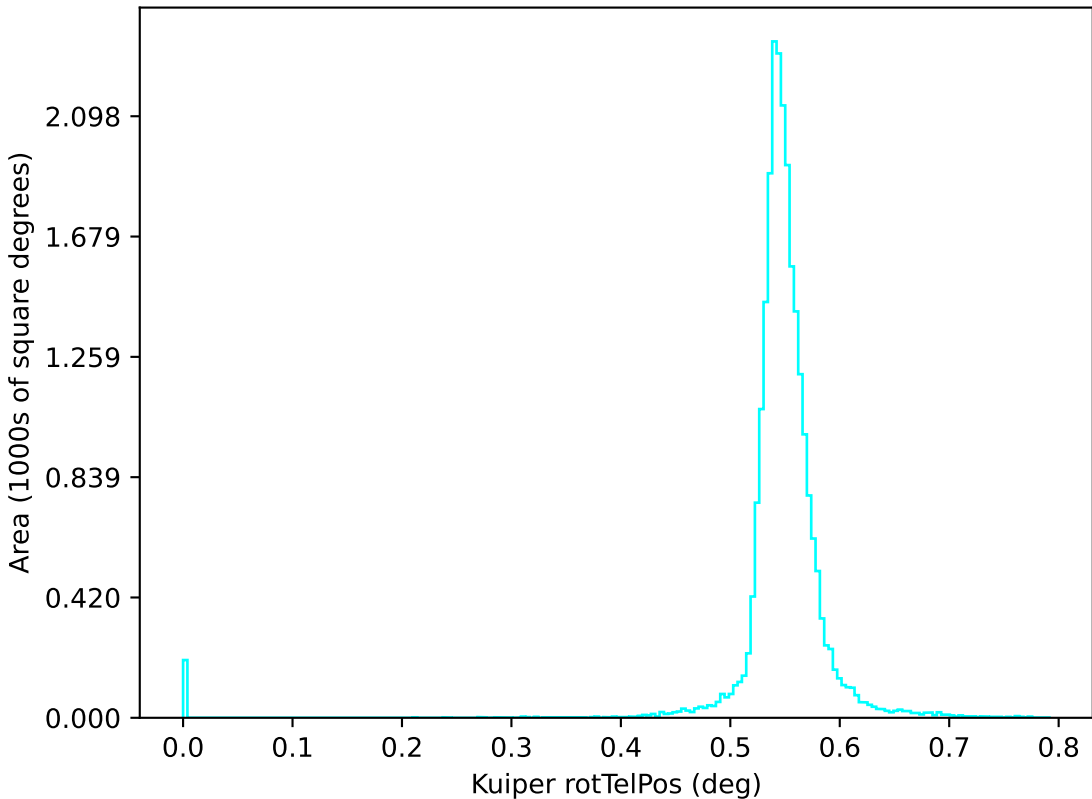
too_combined_s0.8_v3.4_10yrs u: Kuiper rotTelPos
