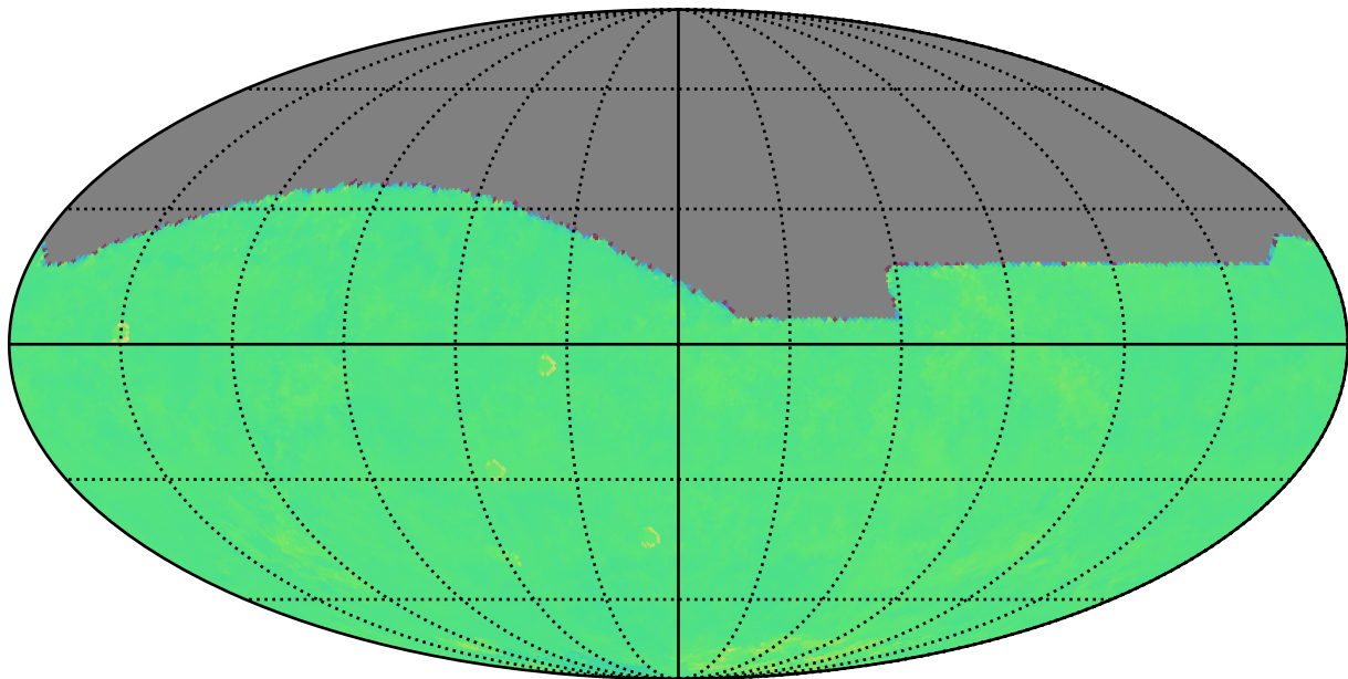
too_combined_s0.8_v3.4_10yrs r: Kuiper rotTelPos
